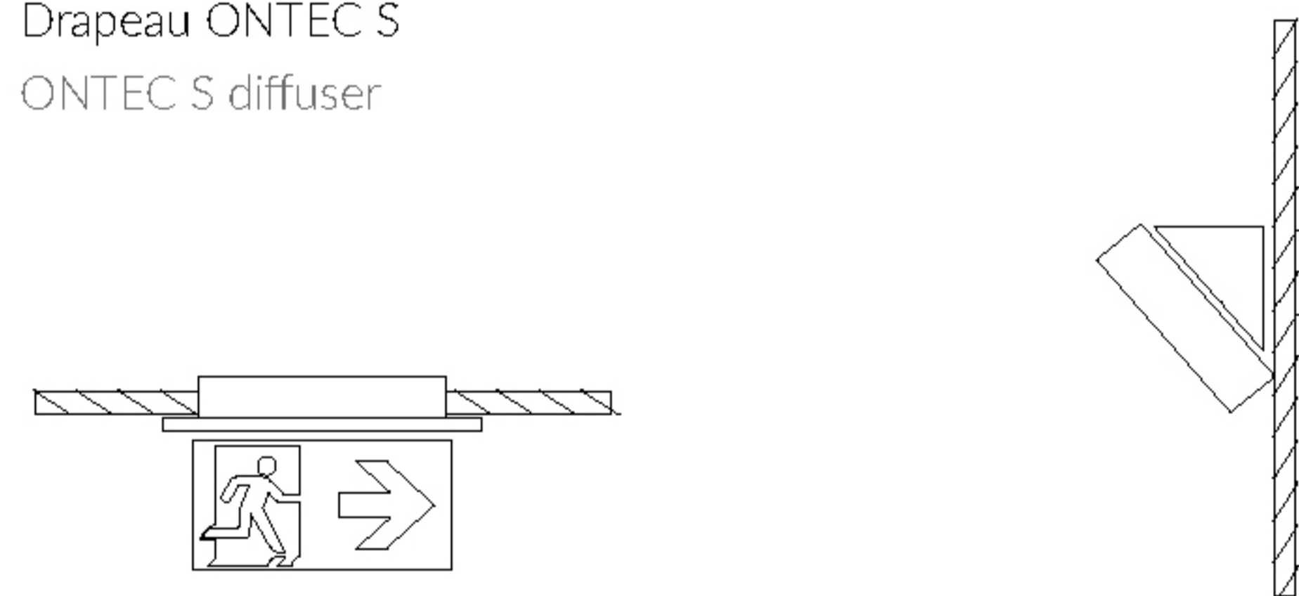
option montage encastré en utilisant le kit option with recessed mount kit applied
